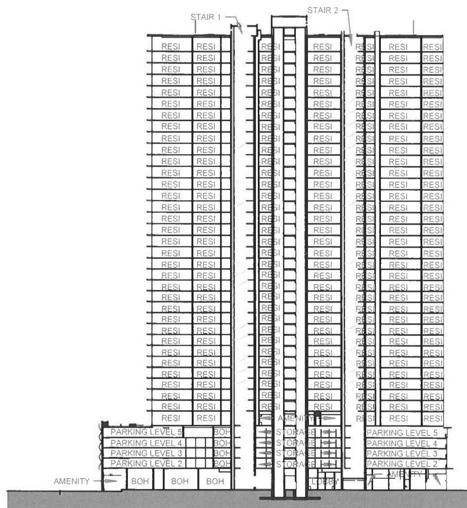
BUILDING SECTION 1
